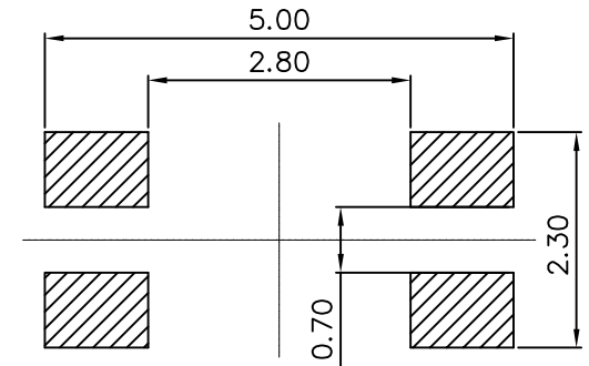
RECOMMENDED P.C.B LAYOUT TOP VIEW (TOLRANCE: \pm 0.05 )
