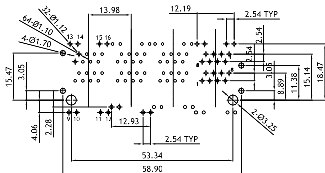
RECOMMENDED P.C.B LAYOUT TOP VIEW (COMPONENT SIDE TOLERANCE±0.05)
