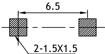
RECOMMENDED P.C.B.LAYOUT ALL TOLERANCES ARE±0.05
