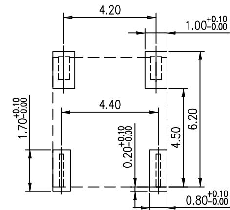
Recommended P.C.Board Layout General Tolerance±0.05
