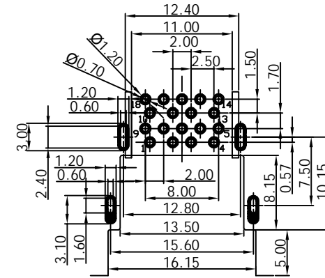
RECOMMENDED P.C.B LAYOUT TOLERANCE: ±0.05(TOP VIEWS)
