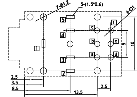
Recommended P.C.B Layout Bottom view, tolerances: ±0.05
