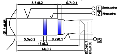
Matching Plug
