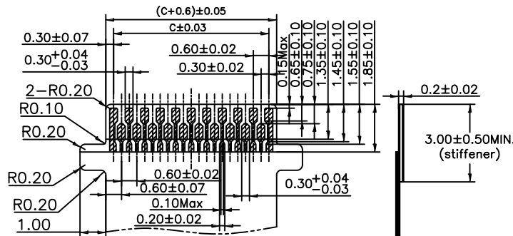
With insertion confirming tabs but lead platings
