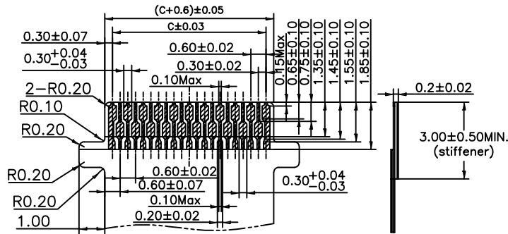
With insertion confirming tabs and lead platings
