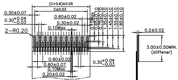
Without insertion confirming tabs but lead platings
