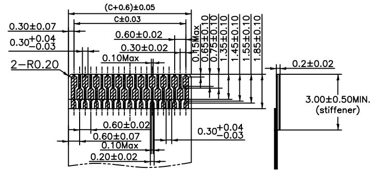
Without insertion confirming tabs and lead platings
