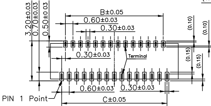
Recommended PCB Layout(Top View) Recommended metal mask pattern(Thickness 0.05mm)
