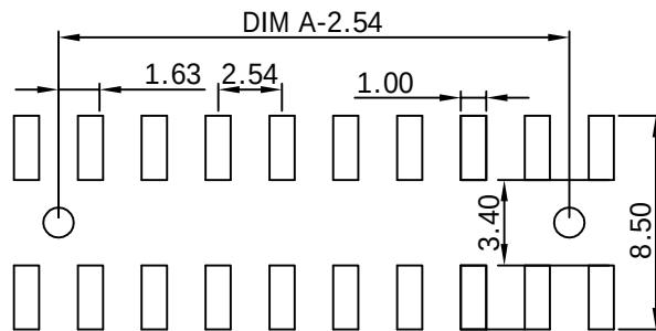
RECOMMENDED P.C.B.LAYOUT ALL TOLERANCES ARE±0.05 W/Plastic Pegs
