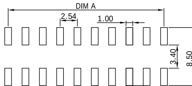
RECOMMENDED P.C.B.LAYOUT ALL TOLERANCES ARE±0.05 W/O Plastic Pegs
