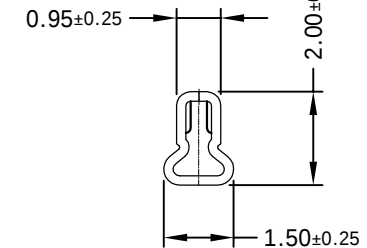
SEC: C-C
