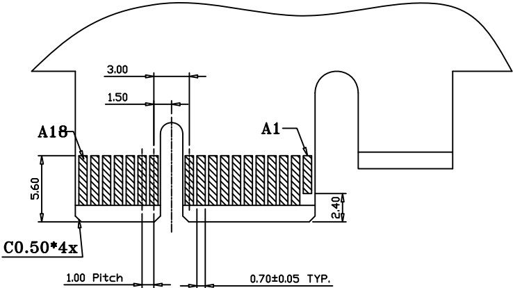
RECOMMENDED EDGE CARD PATTERN(SECONDARY SIDE)
