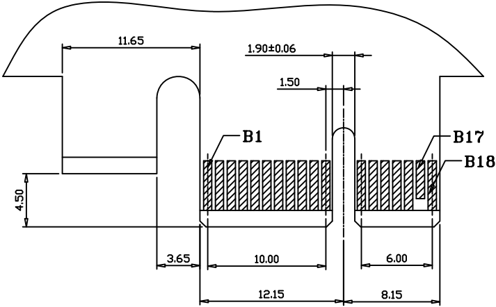
RECOMMENDED EDGE CARD PATTERN(PRIMARY SIDE)
