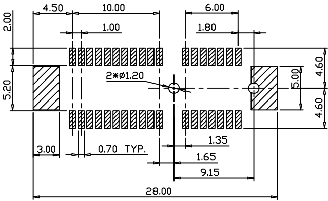
RECOMMENDED PCB LAYOUT (COMPONENT SIDE)TOLERANCE: ±0.05
